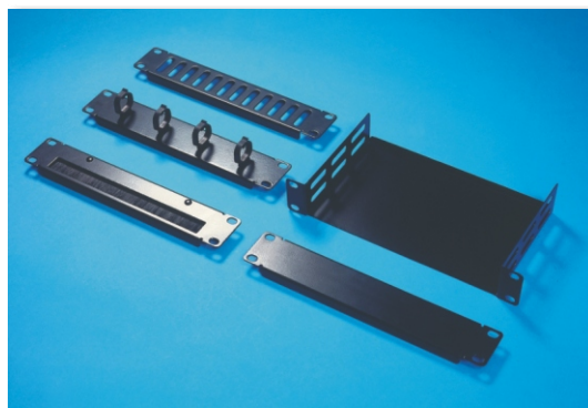
Accessories (clockwise from top) Vent panel, Hub/modem shelf, blank panel, letterbox panel, cable management panel
