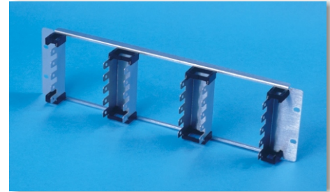
3U Flat Subrack Accepts 15 x 10 pair IDC strips (150 pairs)
