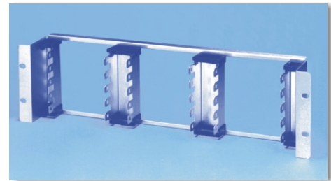
3U Recessed Subrack Accepts 15 x 10 pair IDC strips (150 pairs)
